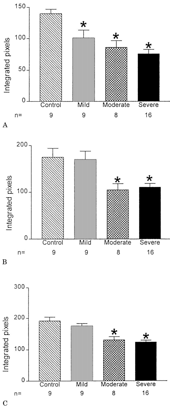
Figure. Dot-blot analysis of the control and AD frontal cortex. (A) Compared with control cases, mild AD cases showed a 25% loss in synaptophysin immunoreactivity. Levels of synaptophysin were further decreased in both moderate and severe cases. (B) Whereas there was no difference in levels of synaptotagmin between control and mild AD cases, there was a significant reduction in levels of immunoreactivity in moderate and severe AD. (C) Levels of growth-associated protein 43 (GAP43) were unchanged in mild AD cases compared with control subjects. In contrast, mild and moderate cases showed a significant and progressive reduction in levels of GAP43 immunoreactivity. *Indicates p < 0.05 (one-way analysis of variance with post hoc Dunnett's test).
